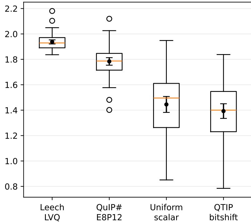
SQNR bits
