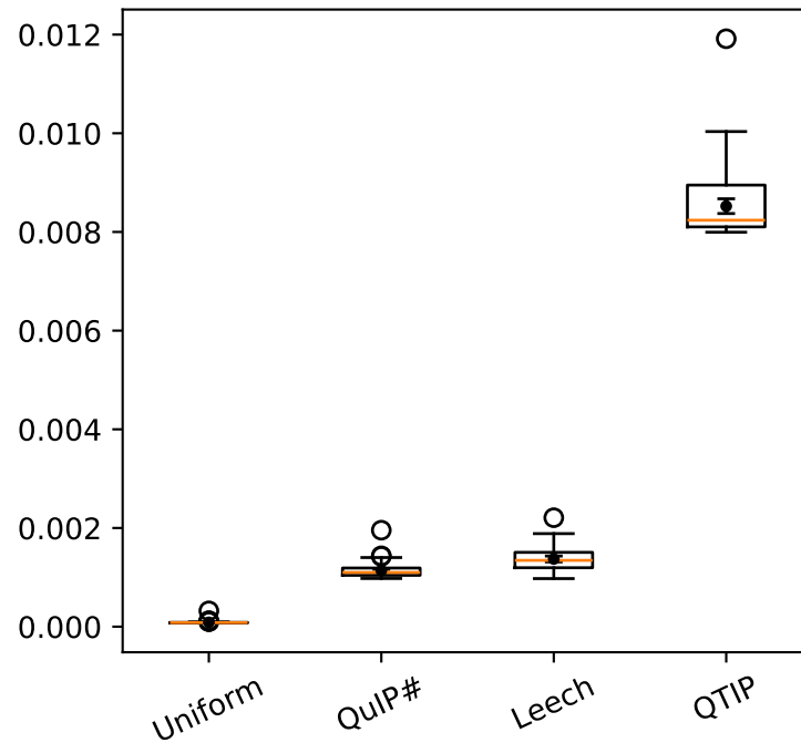
Quantize seconds
