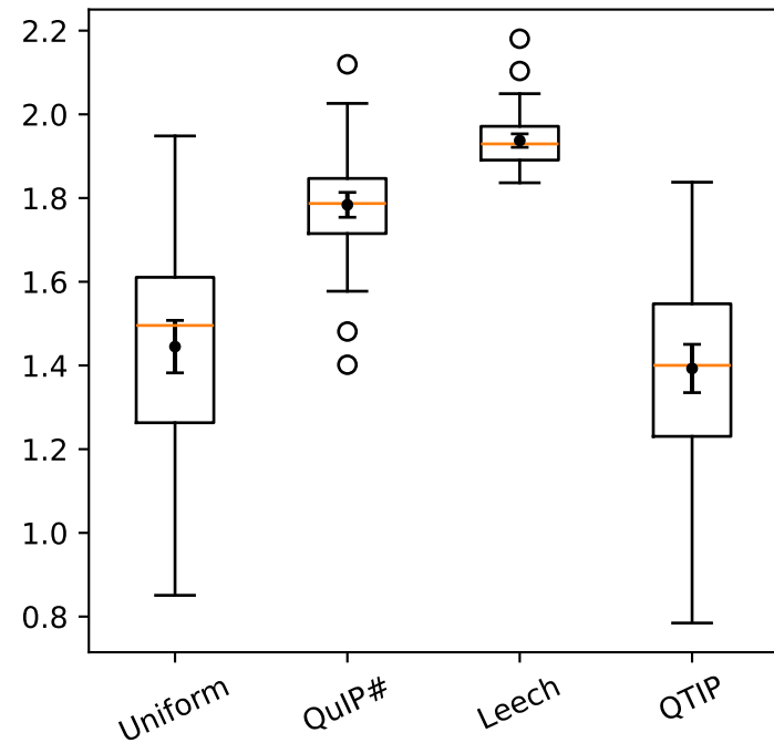
SQNR bits
