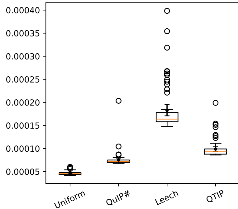
Dequantize seconds
