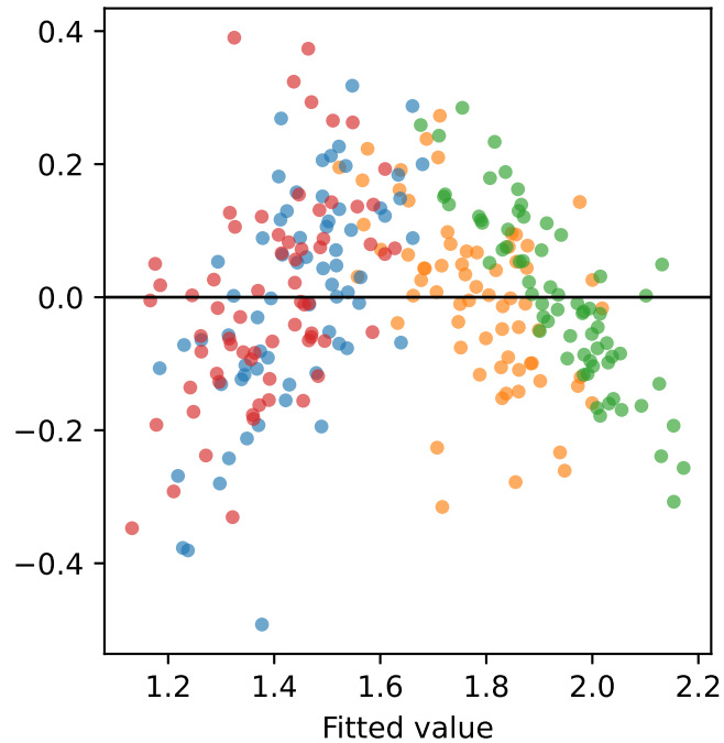
SQNR bits
