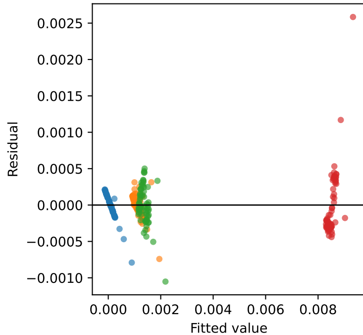
Quantize seconds
