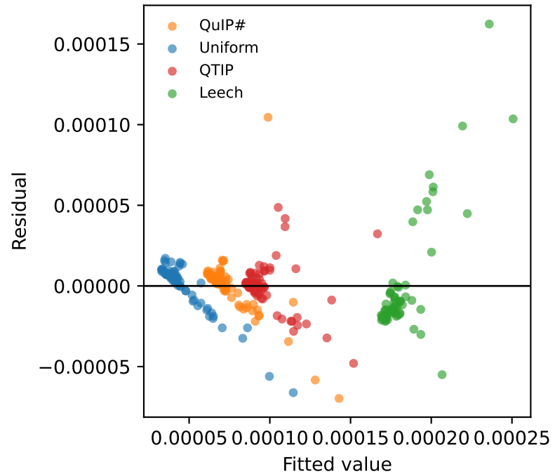
Dequantize seconds
