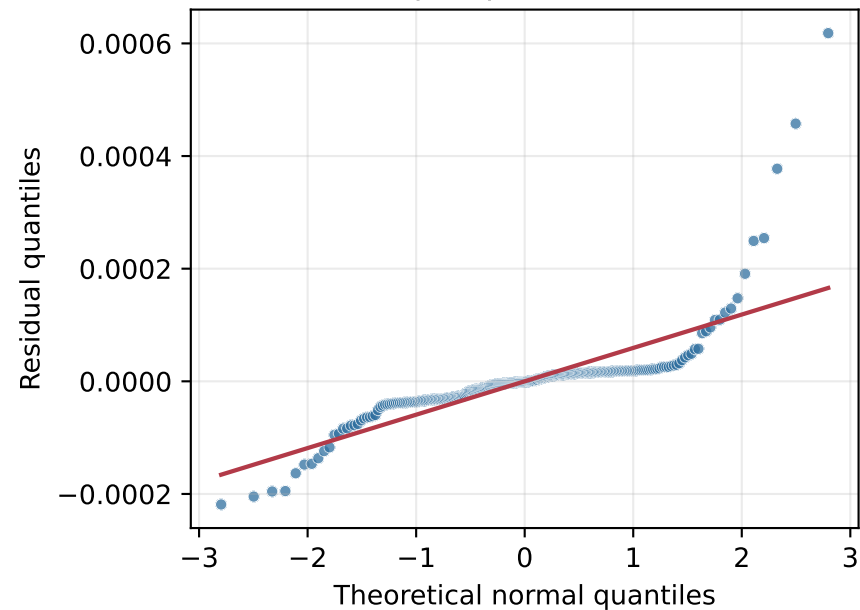
Dequantize seconds Shapiro p = 2.32e-23
