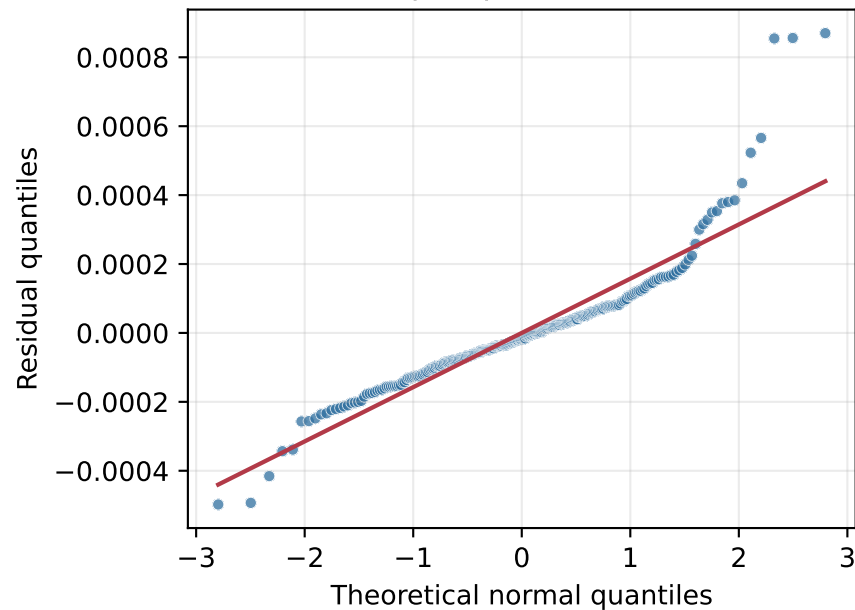
Quantize seconds Shapiro p = 1.74e-14
