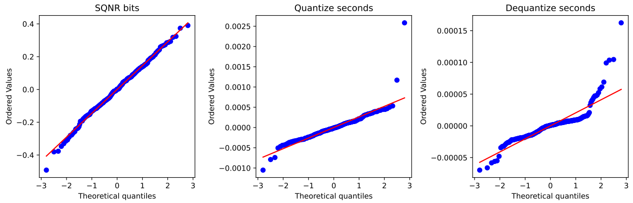
Figure 2: Normal Q-Q plots of ANOVA residuals for the three primary metrics.
