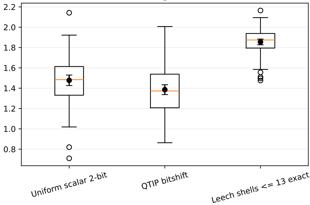
Quantize seconds (lower is better)
