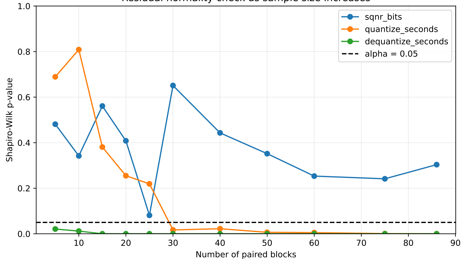
Residual normality check as sample size increases
