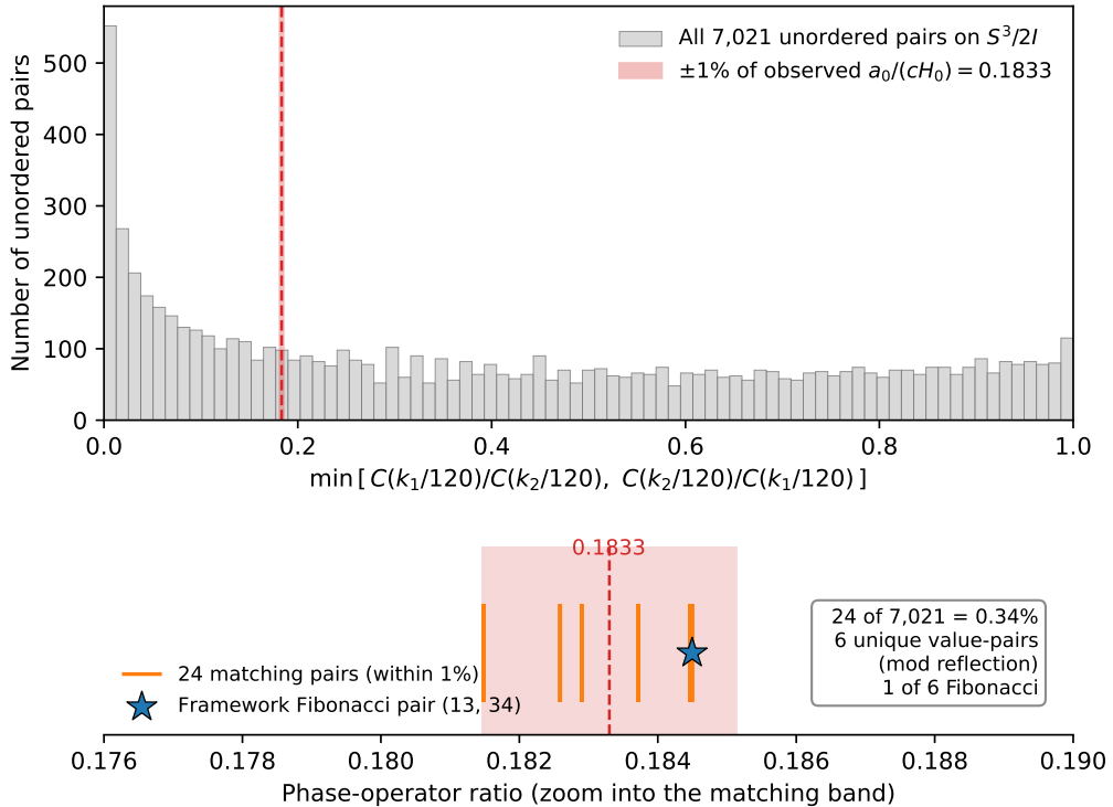
Figure 2.1: Milgrom-ratio sparsity on the 120-domain. Of 7,021 unordered nonzero phase-position pairs, 24 reproduce the observed a_0 / (c H_0) = 0.1833 within 1%; reflection symmetry C(k) = C(120 - k) collapses these to 6 unique phase-operator value pairs. Within the framework's Fibonacci-well subset \{13, 21, 34, 55\}/120 , only the pair (13, 34) matches, marked with a star.
