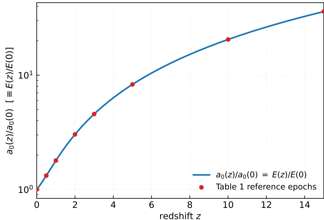
Figure 1: a_0(z)/a_0(0) from z = 0 to z = 15 (flat \Lambda CDM, Planck 2018)
