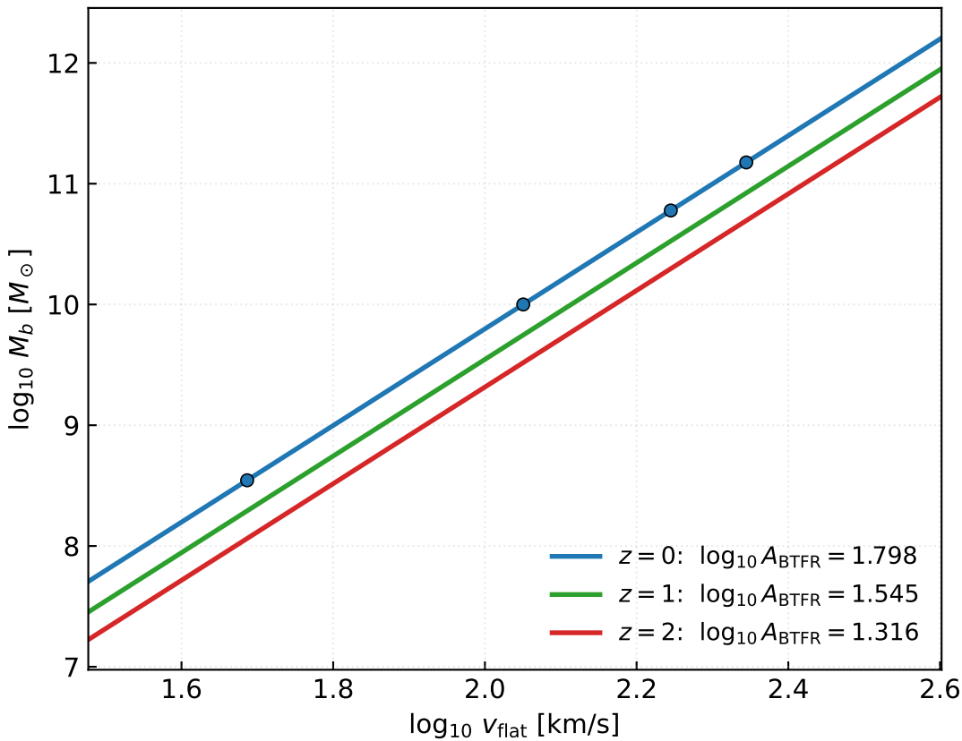
Figure 2: BTFR loci at z = 0, 1, 2 (slope 4, deep-MOND limit)
