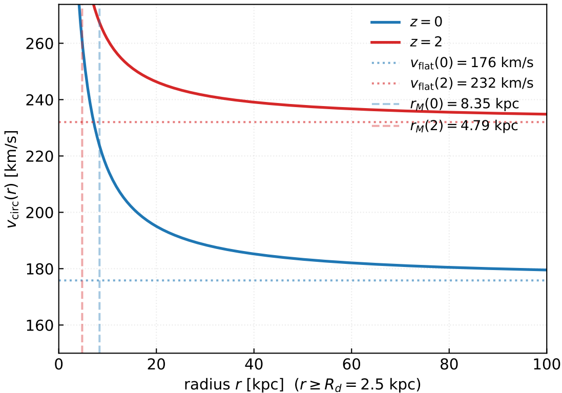
Figure 3: L^* rotation curve at z = 0 and z = 2 (simple MOND, point-mass)
