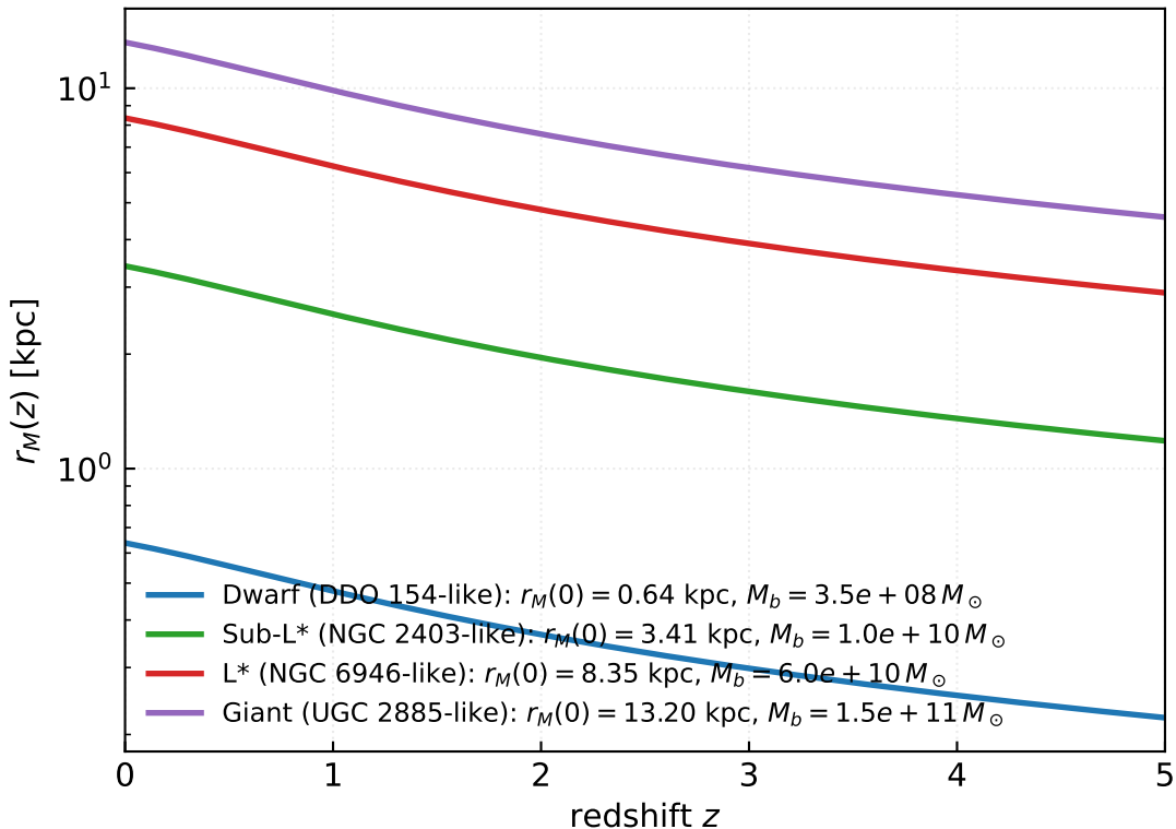
Figure 4: MOND transition radius r_M(z) vs z across galaxy mass
