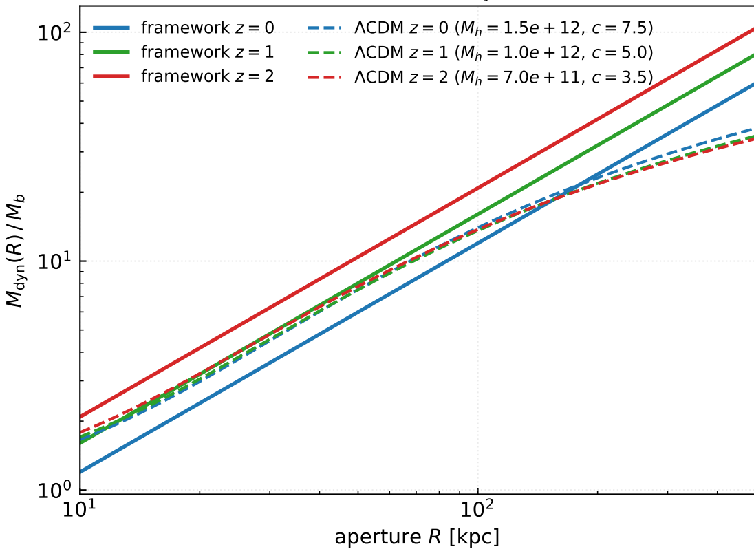
Figure 5: L^* (M_b = 6 \times 10^{10} M_\odot) M_{\text{dyn}}/M_b vs R at z = 0, 1, 2
