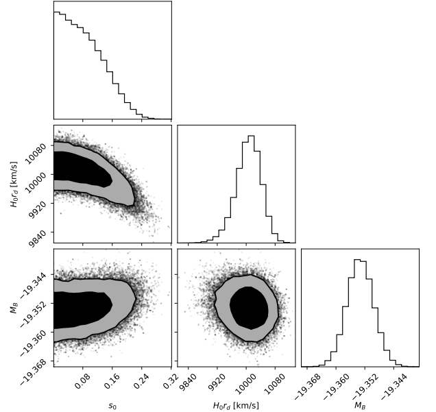
FIG. 3. Corner plot of the Acos posterior in (s_0, H_0 r_d, M_B) space from the SN+BAO fit.
