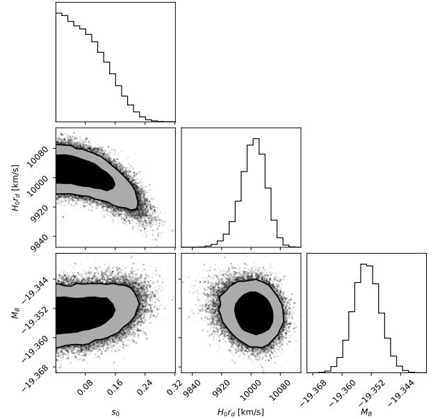
FIG. 3. Corner plot of the \Lambda\text{cos} posterior in (s_0, H_0 r_d, M_B) space from the SN+BAO fit.
