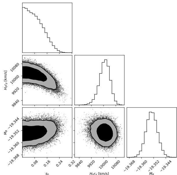
FIG. 3. Corner plot of the Acos posterior in (s_0, H_0 r_d, M_B) space from the SN+BAO fit.
