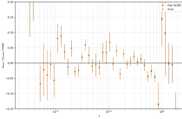
FIG. 4. Pantheon+ binned residuals ( \mu_{\text{data}} - \mu_{\text{model}} ) for \Lambda CDM and \Lambda cos at joint best-fit parameters. The two models are indistinguishable.
