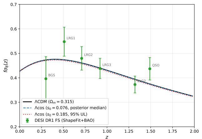
FIG. 5. \Lambda\text{CDM} (solid) and \Lambda\text{cos} f\sigma_{88}(z) trajectories at the posterior median ( s_0 = 0.076 , dashed) and 95\% upper limit ( s_0 = 0.185 , dotted), overlaid with DESI DR1 ShapeFit+BAO growth amplitudes from [16]. The two models are visually indistinguishable at current per-bin precision.
