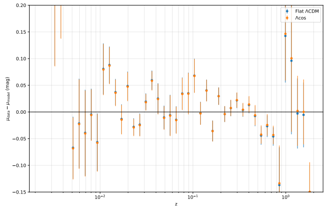
FIG. 4. Pantheon+ binned residuals ( \mu_{\text{data}} - \mu_{\text{model}} ) for \Lambda CDM and \Lambda cos at joint best-fit parameters. The two models are visually indistinguishable in the binned residuals.
