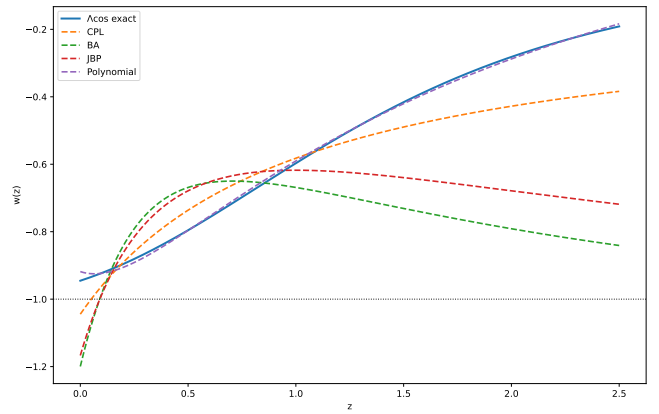
FIG. 1. Exact \Lambda\text{cos} w_{\text{eff}}(z) (solid, always > -1 ) overlaid with recovered w(z) from all four parameterizations. CPL, BA, and JBP dip below w = -1 at low z . The three-parameter polynomial tracks the true curve without crossing.
