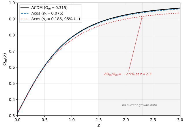
FIG. 6. \Omega_m(z) diagnostic for \Lambda CDM and Acos at the 95% upper limit ( s_0 = 0.185 ). The 2.9% split at z = 2.3 is beyond the reach of current growth data but accessible to next-generation surveys.
