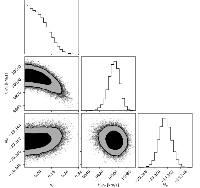
FIG. 3. Corner plot of the \Lambda cos posterior in (s_0, H_0 r_d, M_B) space from the SN+BAO fit.
