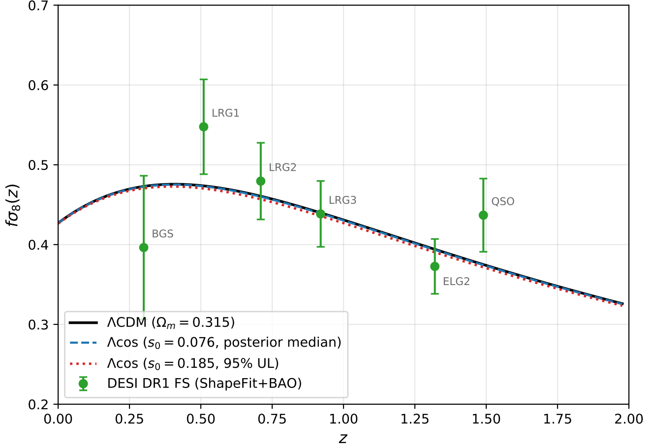
FIG. 5. \Lambda CDM (solid) and \Lambda cos f\sigma_{s8}(z) trajectories at the posterior median ( s_0 = 0.076 , dashed) and 95% upper limit ( s_0 = 0.185 , dotted), overlaid with DESI DR1 ShapeFit+BAO growth amplitudes from [18]. The two models are visually indistinguishable at current per-bin precision.
