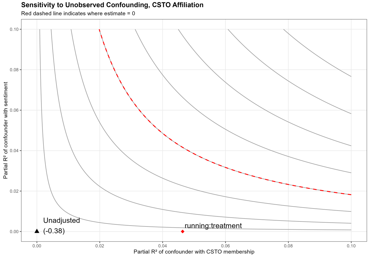
Figure 8: Sensitivity of the \text{CSTO} \times \text{treatment} interaction to unobserved confounding, following Cinelli and Hazlett (2020). The red dashed line indicates the combinations of confounder strength that would reduce the estimate to zero. The triangle marks the unadjusted estimate; the diamond marks the benchmark covariate ( running:treatment ).
