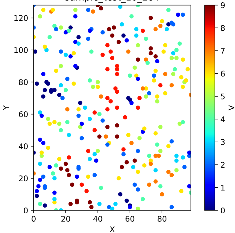
sample_test_10_284
