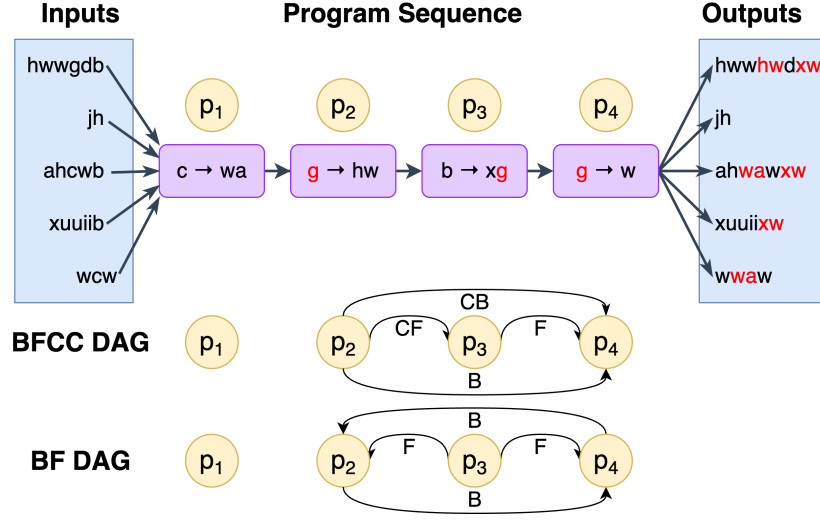
Figure 5: A PBEBench data instance. The model receives input-output word pairs from an unknown cascade of rewrite rules and must produce a Python program implementing those rules. Labels B, F, CB, and CF (not visible to the model) indicate the ordering relation between successive rules.
