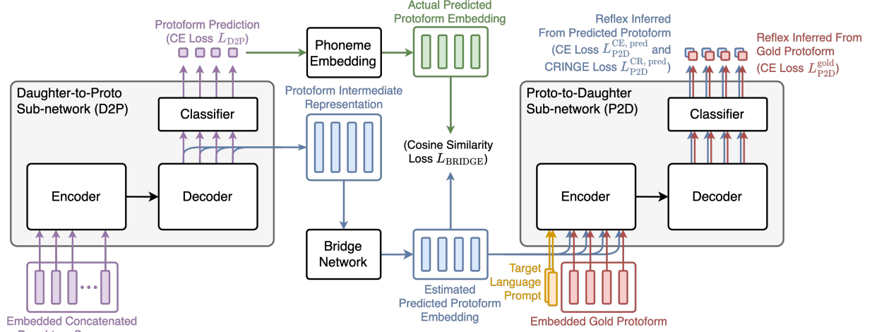
Figure 2: The D2P2D architecture. The D2P sub-model encodes cognate sets as protoforms; the bridge network maps D2P decoder output to estimated protoform embeddings; the P2D sub-model decodes those embeddings back into reflexes. When labeled protoforms are available, gold embeddings supervise the bridge via a cosine similarity loss.
