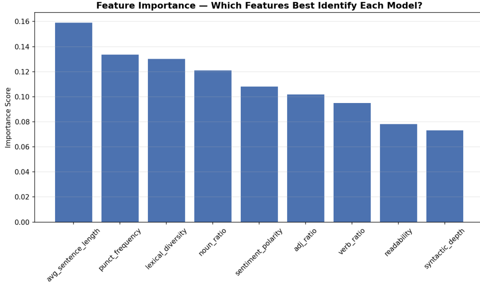
Figure 5: Feature importance scores from Random Forest classifier.
