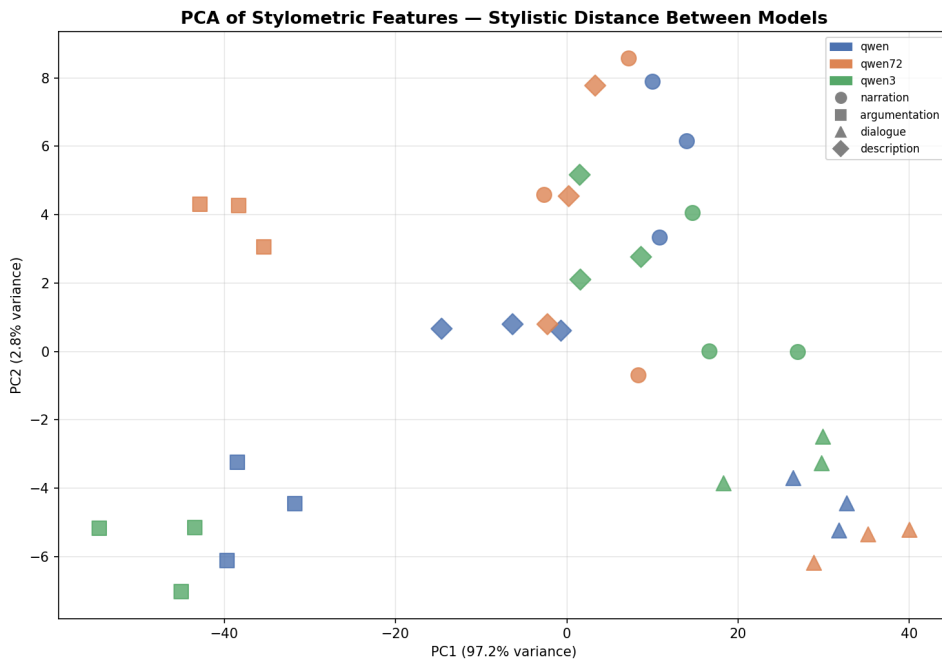
Figure 2: PCA of stylistic features. PC1 explains 97.2% of variance. Points represent individual texts; colors indicate model identity; shape indicate writing genre.
