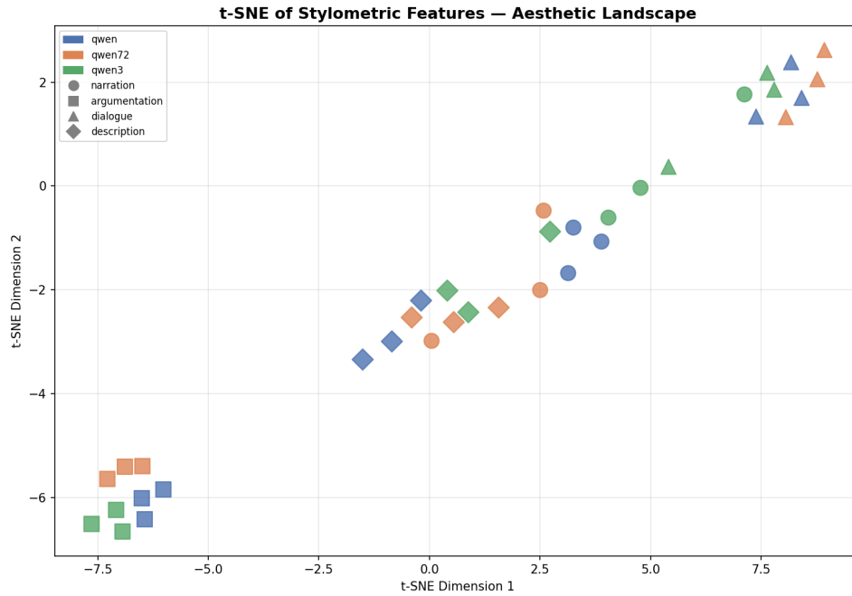
Figure 3: t-SNE aesthetic landscape of stylometric embeddings. Four distinct genre clusters emerge, with dialogue and argumentation showing the clearest separation.
