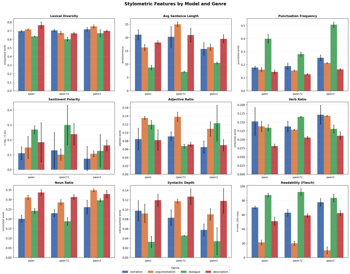
Figure 1: All nine stylometric features by model and genre. Error bars show standard deviation across 3 repetitions.
