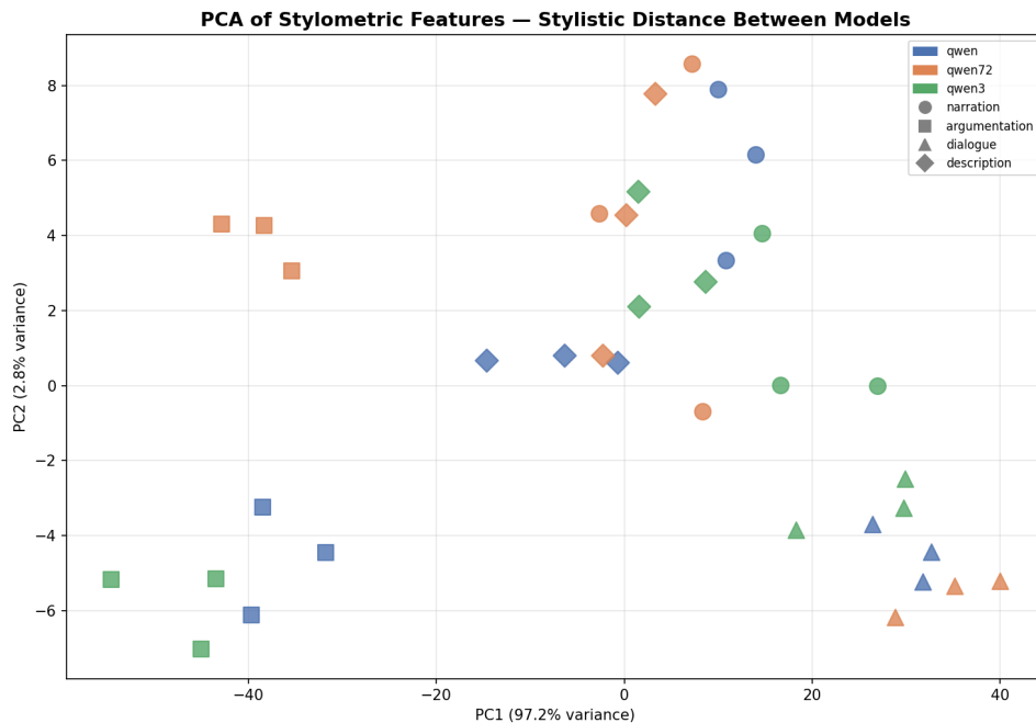
Figure 2: PCA of stylometric features. PC1 explains 97.2% of variance. Points represent individual texts; colors indicate model identity; shape indicate writing genre.
