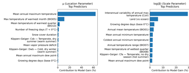
Figure 2. Top predictors of Gumbel distribution parameters by percentage contribution to model gain. Mean annual maximum temperature dominates the location parameter ( \mu ), while interannual variability of annual maximum temperature dominates the scale parameter [ \log(\beta) ].
