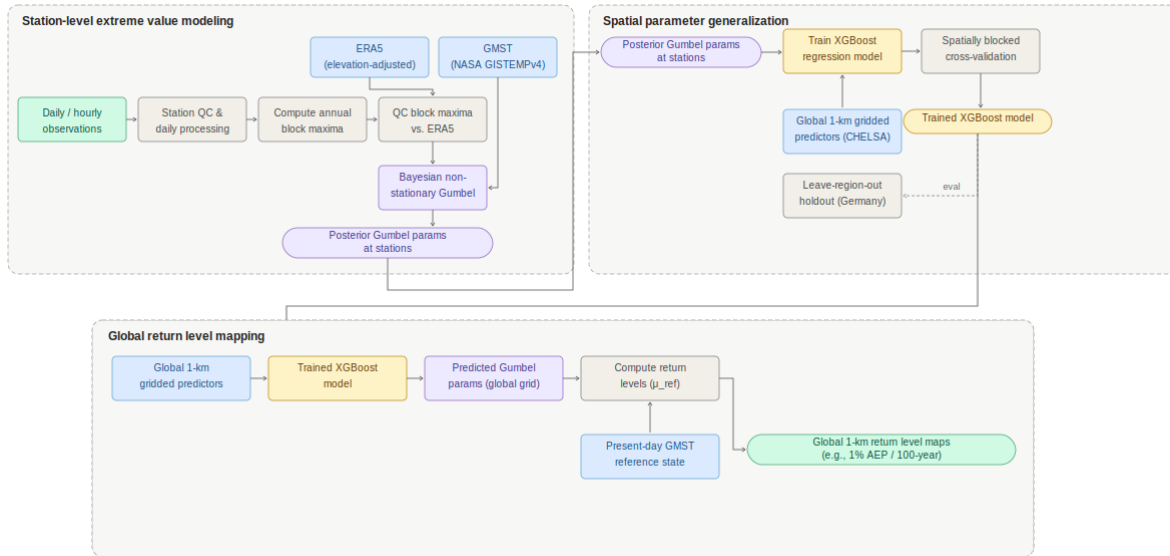
Figure 1. Overview of the three-stage modeling pipeline: (1) station-level non-stationary Gumbel extreme value modeling, (2) spatial parameter generalization via XGBoost, and (3) global return level mapping at 1-km resolution.
