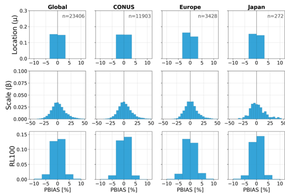
Figure 3. Comparison of percentage bias (PBIAS) for Gumbel location ( \mu ), scale ( \beta ), and the 1% annual exceedance probability return level ( RL_{100} ) across GHCN stations. Panels show the distribution of bias globally and by region. Zero PBIAS indicates exact agreement between local and regionalized estimates; negative values signify model underprediction.
