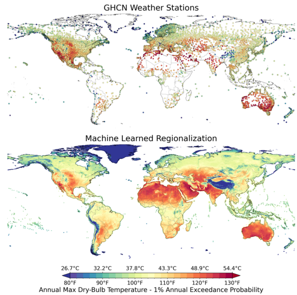
Figure 4. Global distribution of the 1% annual exceedance probability (100-year return level) for annual maximum dry-bulb temperature. The upper panel displays local estimates derived from the Global Historical Climatology Network (GHCN) stations. The lower panel shows the regionalized output produced by the machine learning model, providing spatially complete coverage at 30 arc-seconds ( \sim 1\text{-km} ) resolution.
