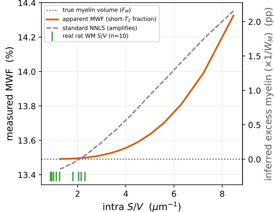
B fine WM reads myelin-rich
