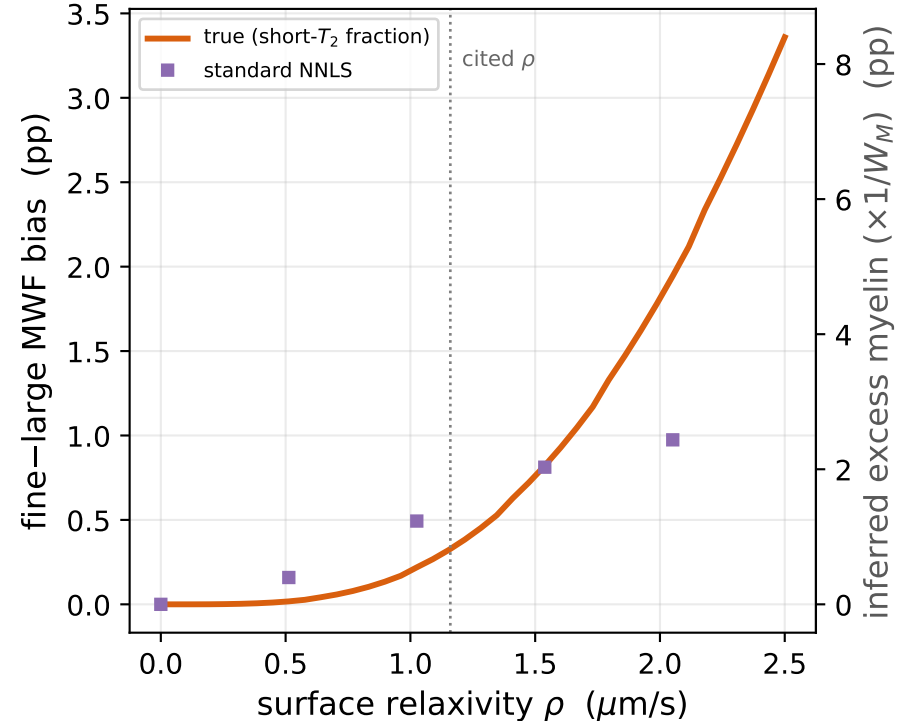
C bias vs the poorly-known \rho
