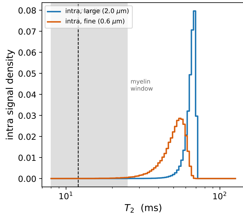
A fine-axon intra T_2 crosses the myelin window
