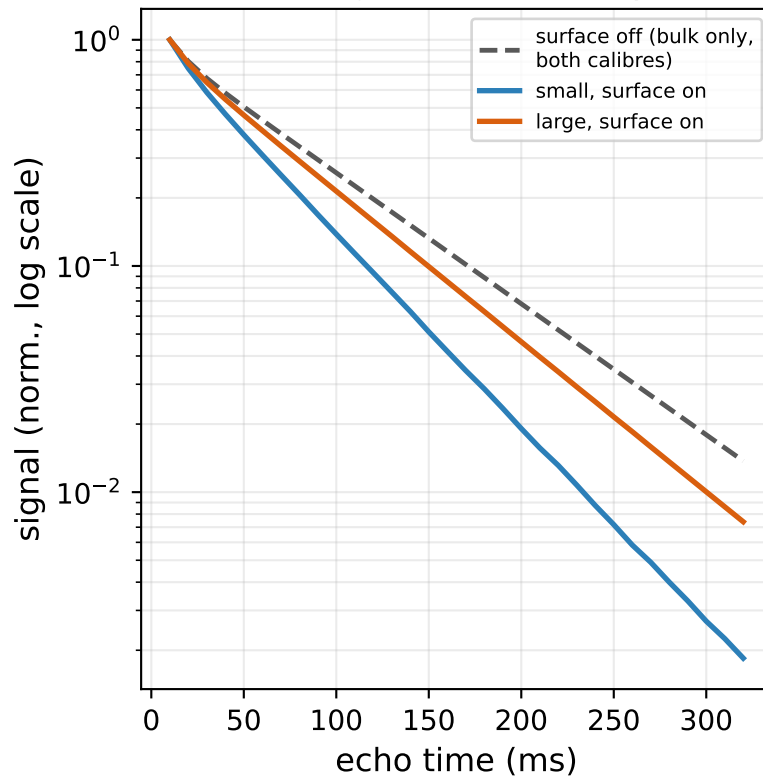
B engine CPMG decay
