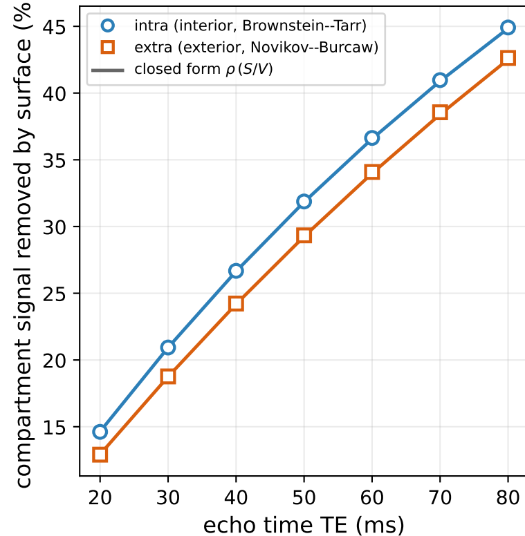
A wall counting reproduces \rho(S/V)
