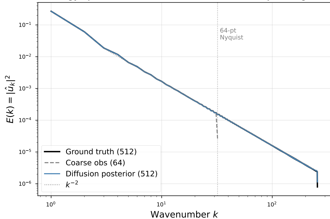
Energy spectrum — resolution 512 (time & traj averaged)
