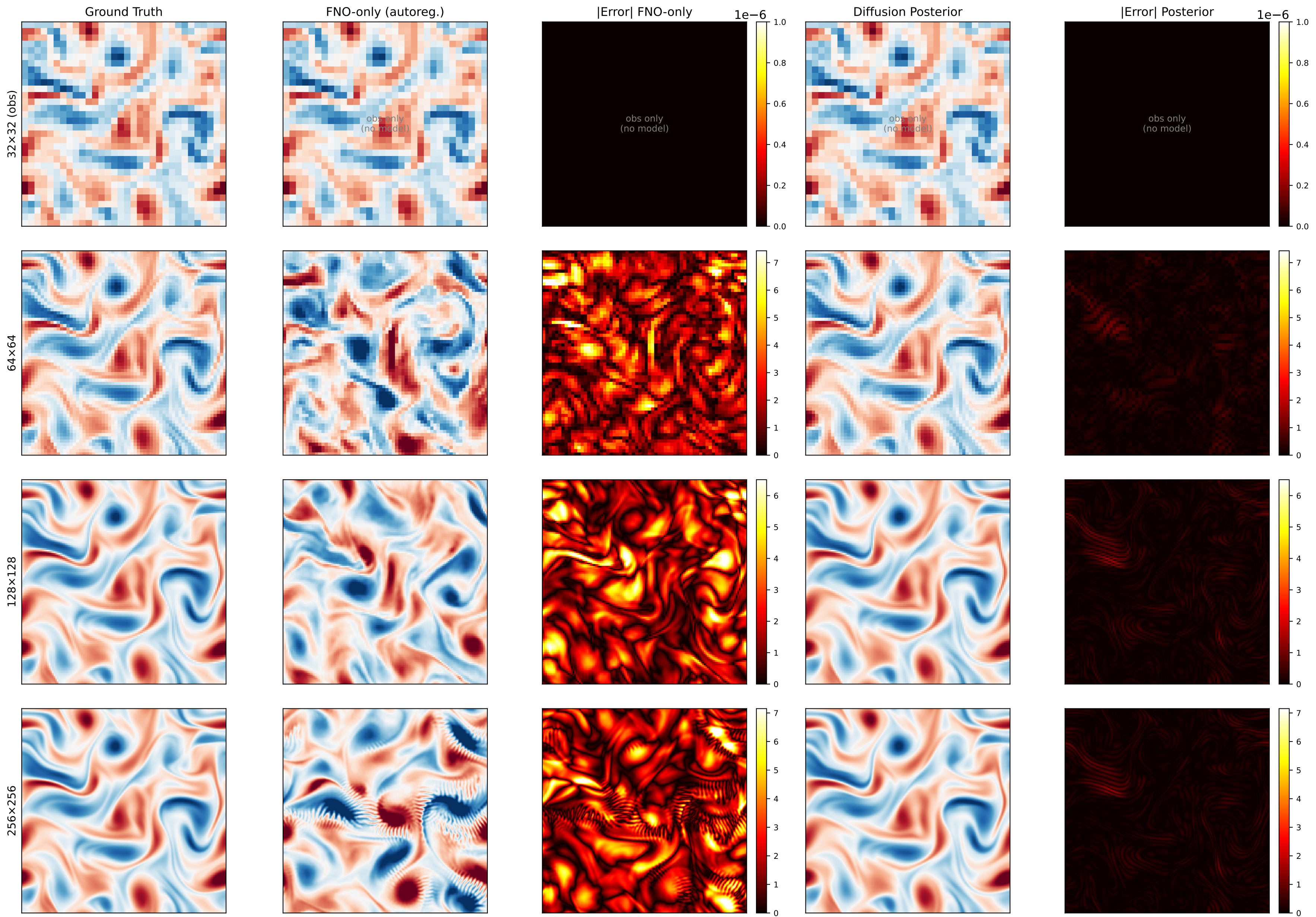
Vorticity Field Comparison | t=50, trajectory 0
