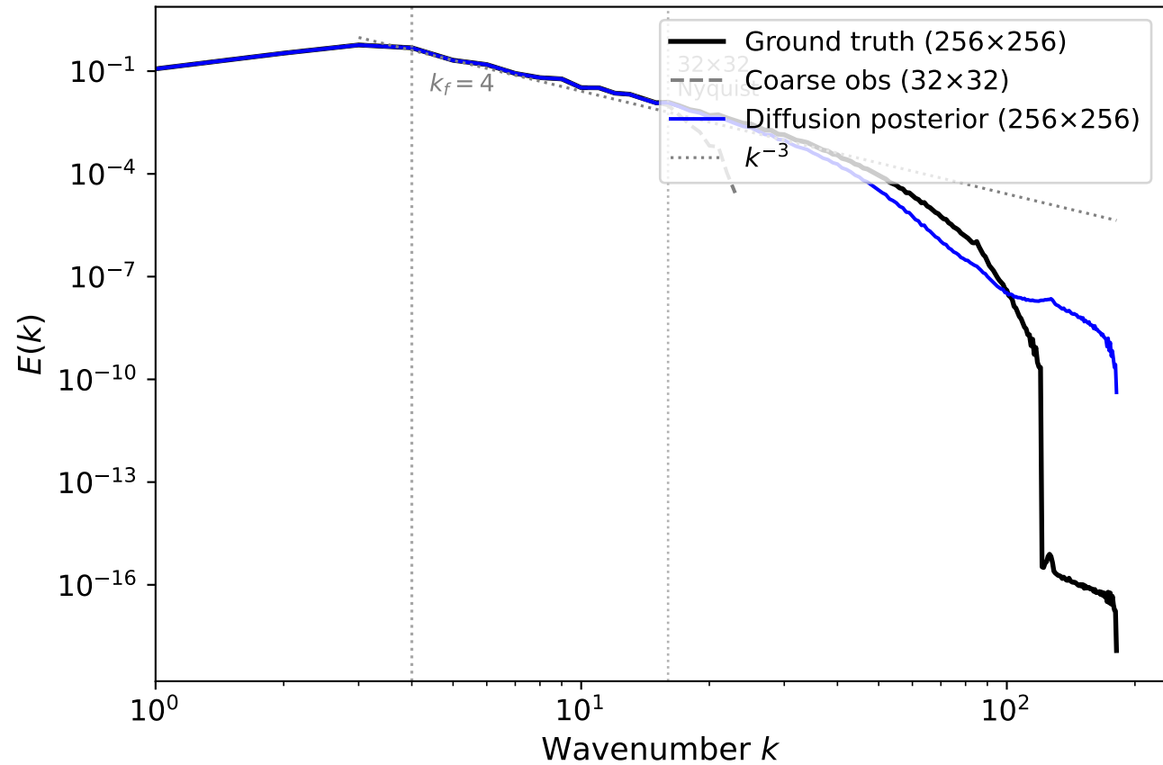
Radial Energy Spectrum (256×256, all time steps & trajectories)
