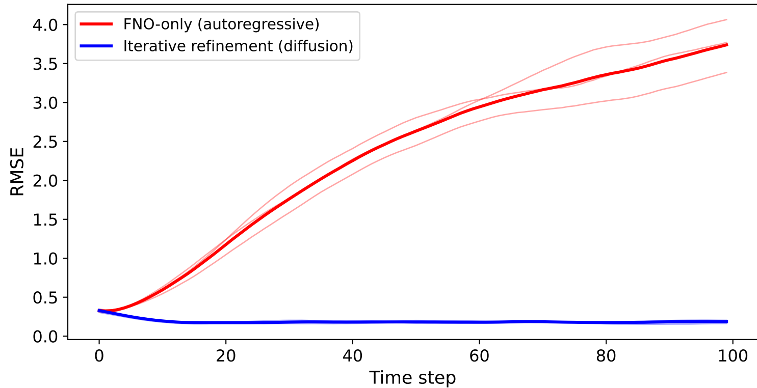
RMSE Over Time (256×256)
