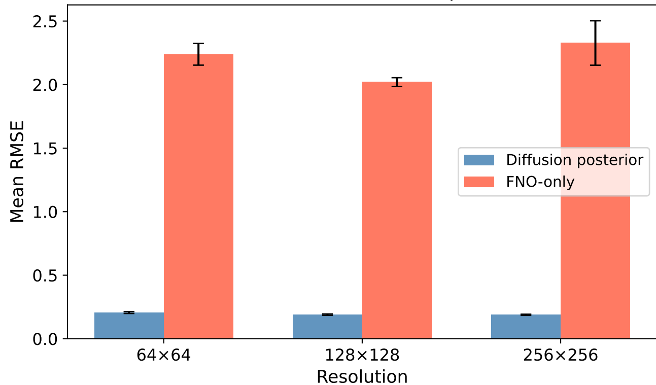
Per-Resolution RMSE Comparison
