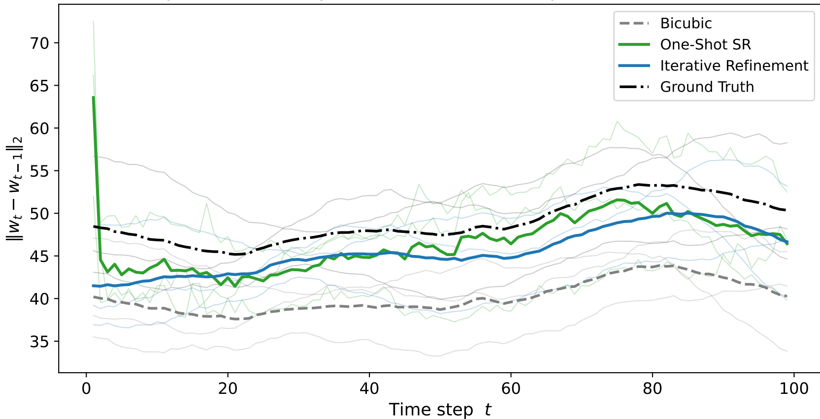
Temporal Consistency (frame-to-frame L2 displacement, 256×256)
