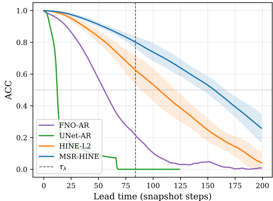
(b) ACC vs. lead time
