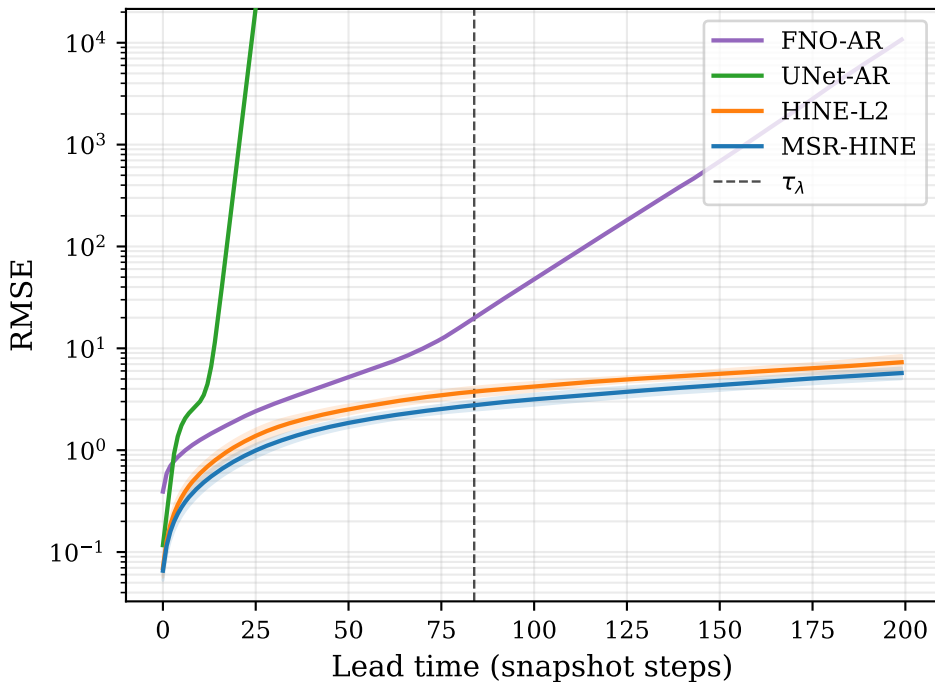
(a) RMSE vs. lead time
