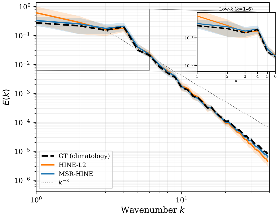
Time-averaged energy spectrum at saturation (steps 160-199, last 20% of rollout)
