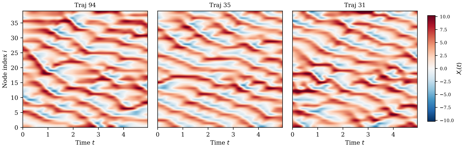
Lorenz-96 (L96, N = 40 , F = 8 ) — sample trajectories
