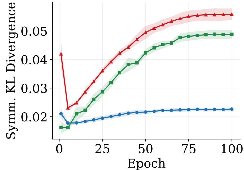
(c) Test Equivariance
