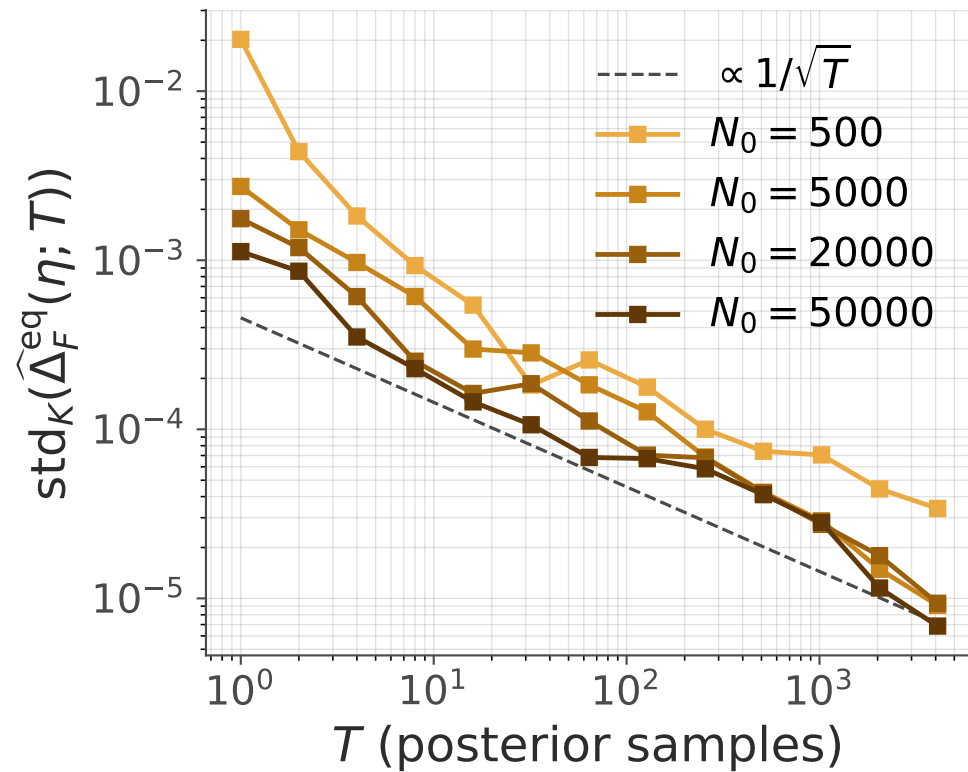
(b) MC complexity
