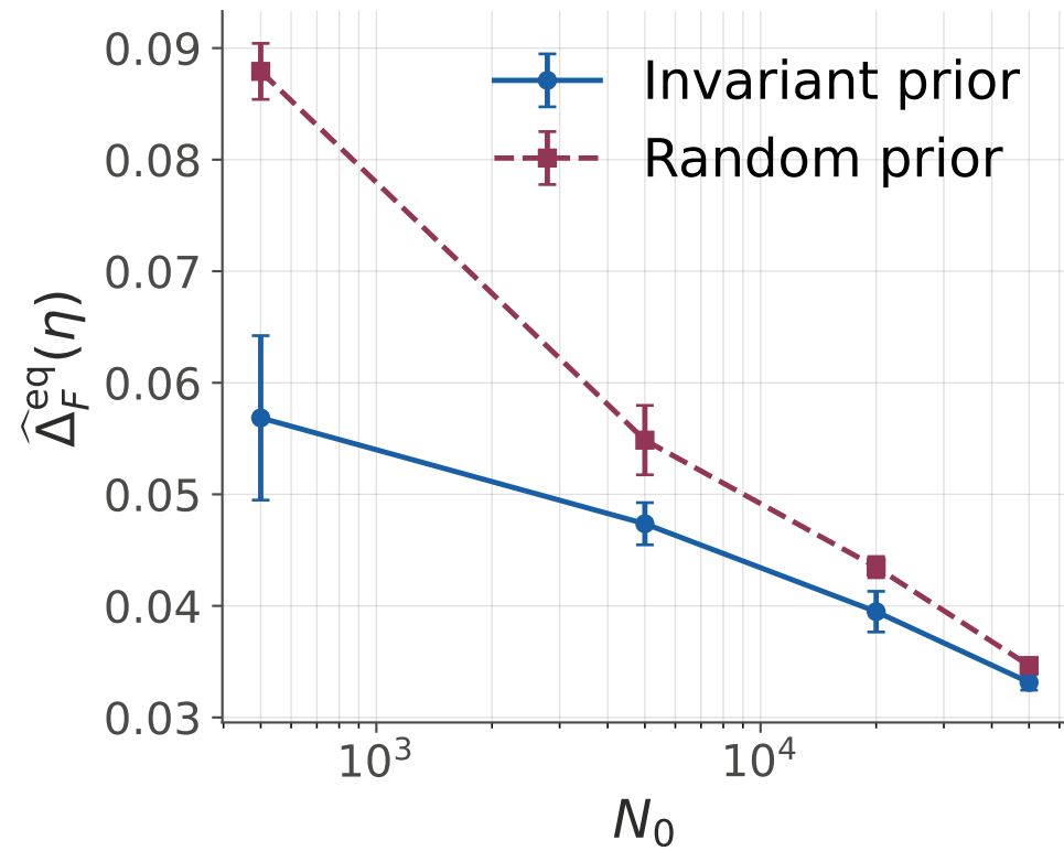
(a) Defect vs. dataset size
