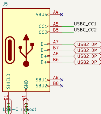
USB-C root to GND
