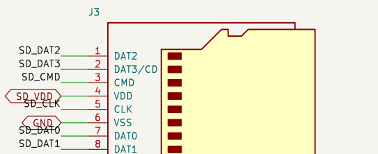
microSD
