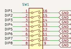
DIP x8
