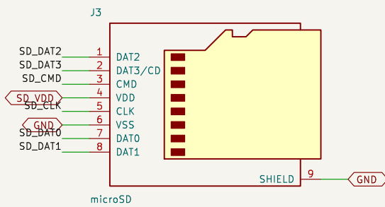
microSD
