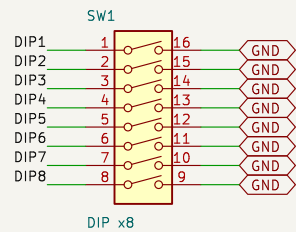
DIP x8
