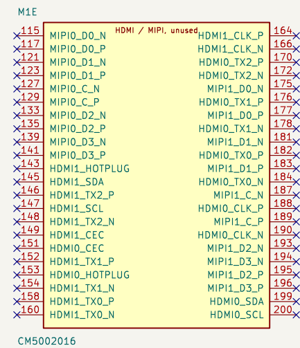
CM5002016
