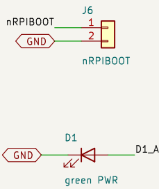
nRPIBOOT
