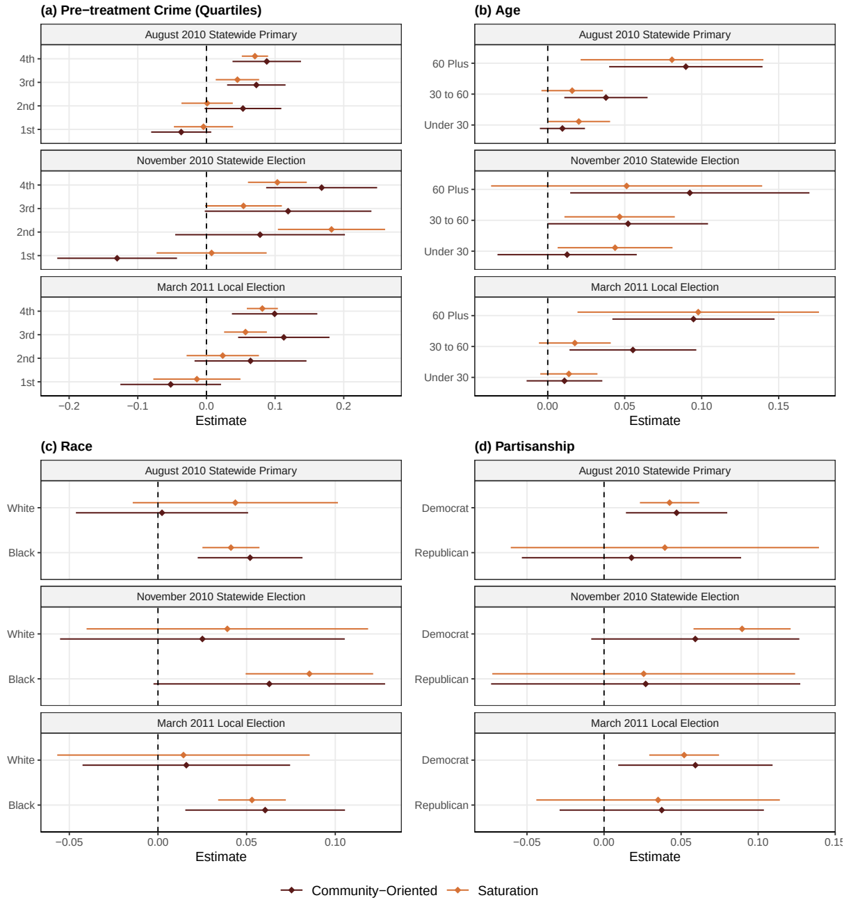
Figure 3: Heterogeneous Effects
