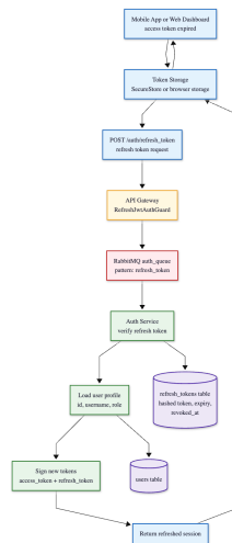
Figure 4.5: Refresh token rotation sequence for renewing access tokens and invalidating old refresh tokens.
