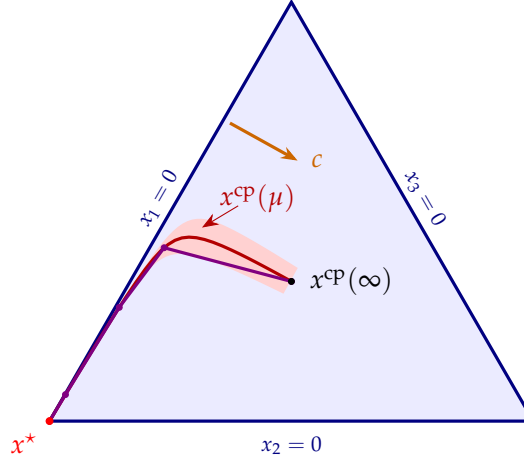
Figure 2: Path following in a tube, computed exactly for the LP \min x_1 + \varepsilon x_2 + \varepsilon^2 x_3 over the simplex x_1 + x_2 + x_3 = 1, x \geq 0 , with \varepsilon = 1/50 , drawn via the isometric embedding of the plane \{x \in \mathbb{R}^3 : x_1 + x_2 + x_3 = 1\} into \mathbb{R}^2 . The feasible region becomes an equilateral triangle whose edges are the facets x_i = 0 , and each slack x_i is proportional to the distance to the corresponding edge, with the same constant for all three. The red curve is the central path, running from the analytic center x^{\text{CP}}(\infty) = (\frac{1}{3}, \frac{1}{3}, \frac{1}{3}) — the centroid of the triangle — to the optimal vertex x^* = e_3 ; the shaded region is the multiplicative tube of factor 1.1: all points whose three slacks are within a factor 1.1 of the slacks of the central path point with the same optimality gap. The violet curve is a piecewise linear path from x^{\text{CP}}(\infty) to x^* staying inside the tube, with T = 4 segments (chosen greedily); its last segment reaches x^* along the asymptotic direction of the path. The tube is wide where the path is straight and pinches at the elbows — near the elbows is where segments are spent.
