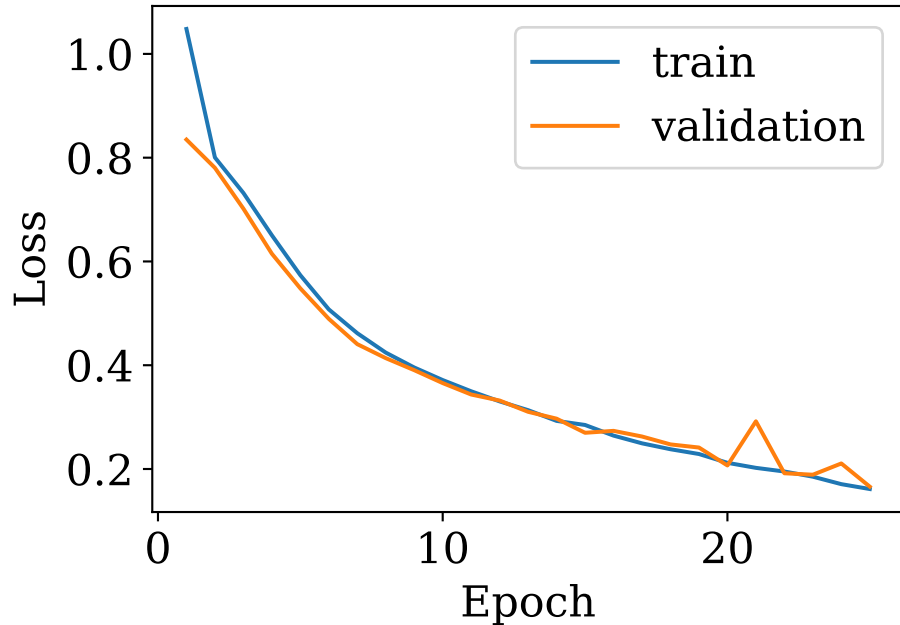
Loss
