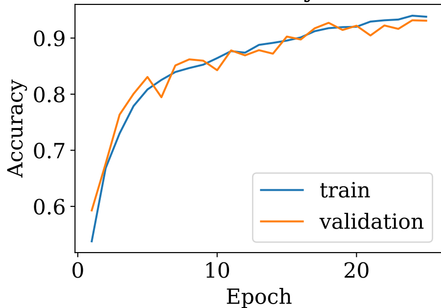
Accuracy
