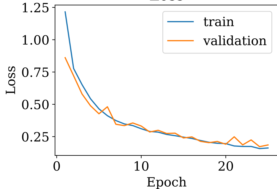
Loss
