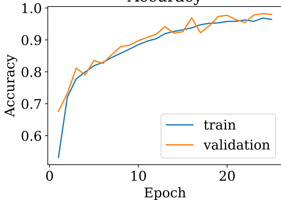
Accuracy
