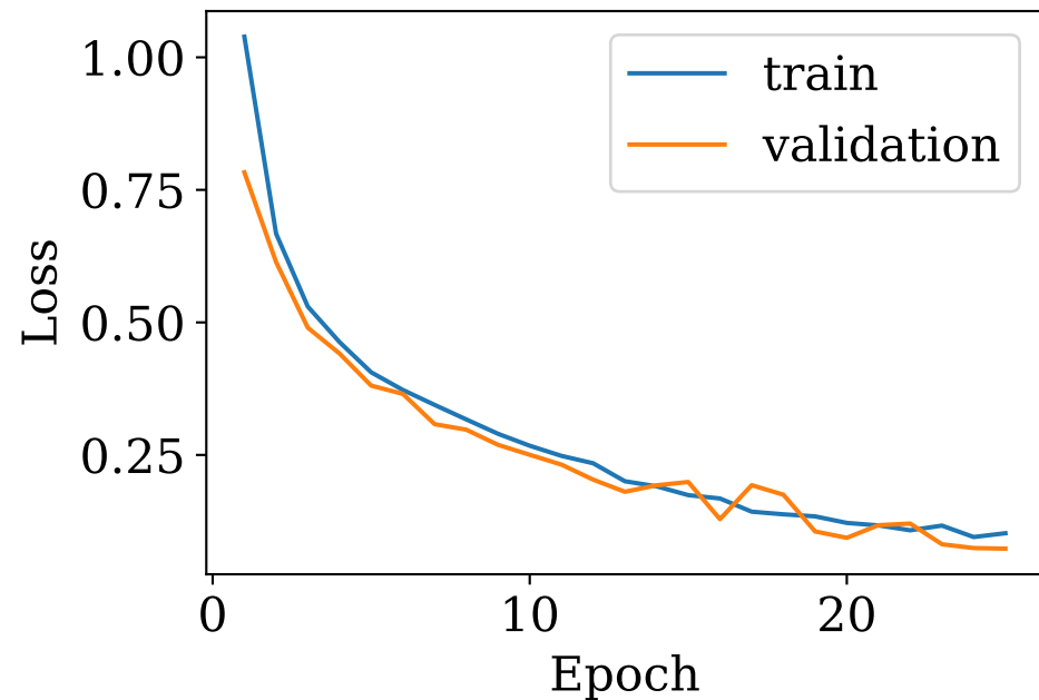
Loss
