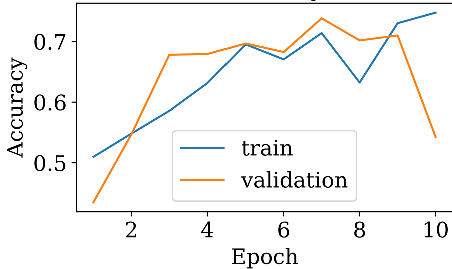
Accuracy
