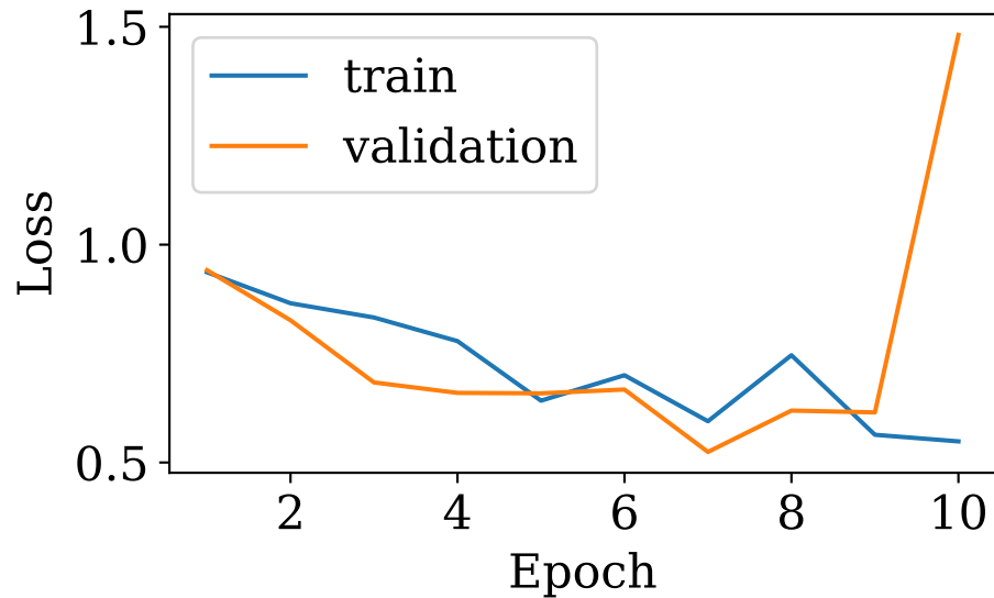
Loss
