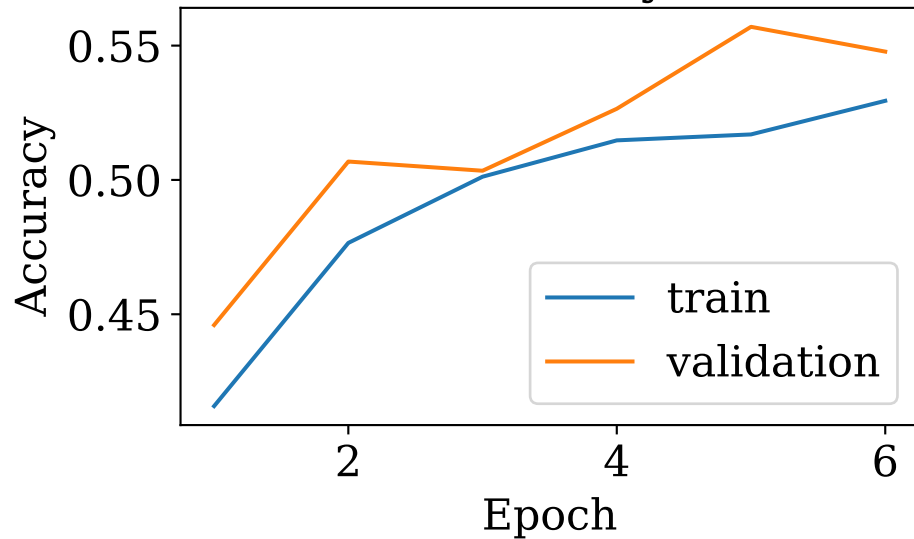
Accuracy
