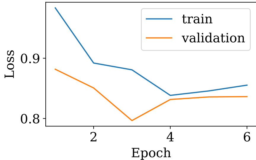
Loss
